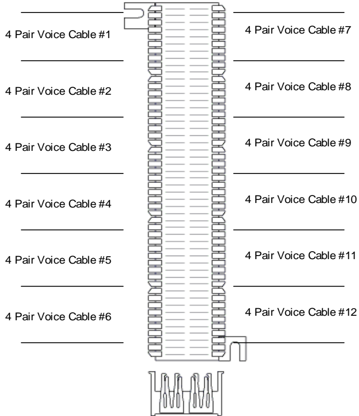
Fig 5. VOICE TERMINATION - S66-M1 50 PAIR BLOCK
