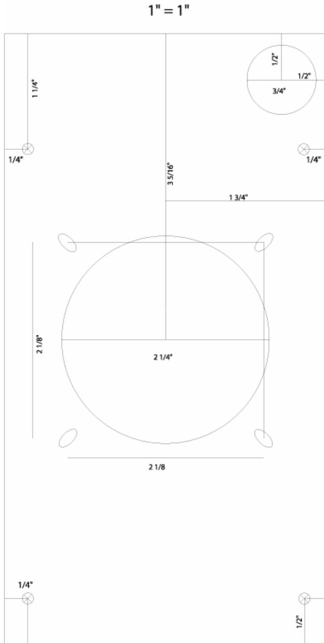
Figure 9 – Elevator Telephone Template
