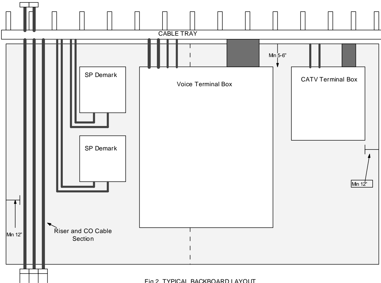
Fig 2. TYPICAL BACKBOARD LAYOUT
