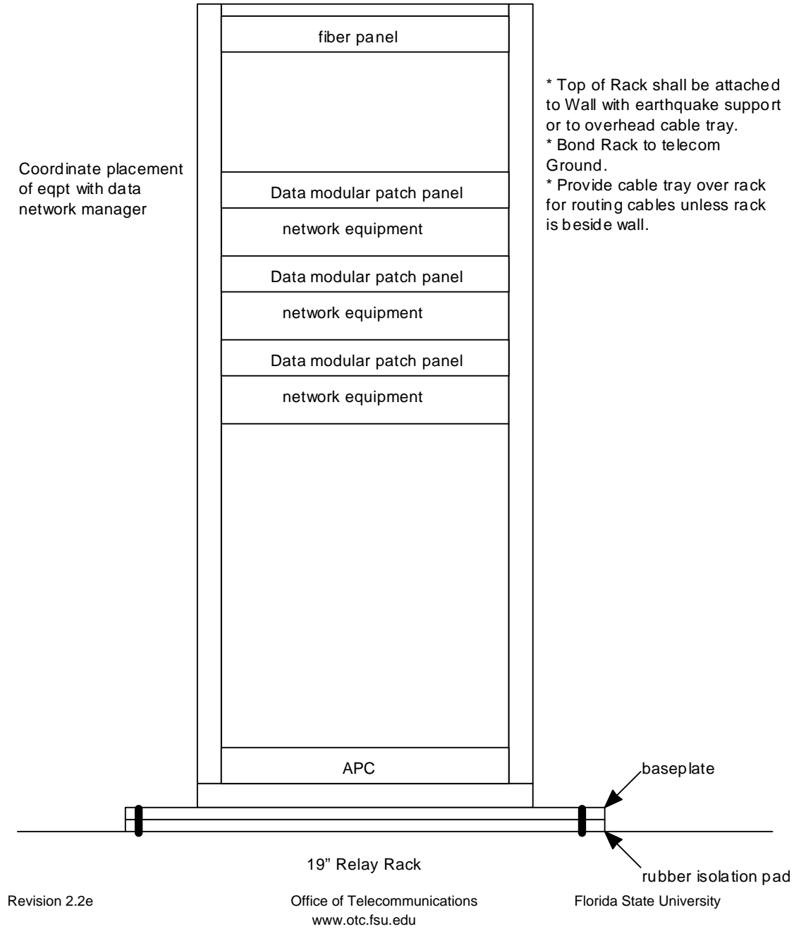
Fig 8. Typical Relay Rack Layout
