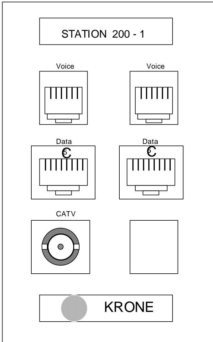
Office of Telecommunications Florida State University Fig 6. Krone Faceplate Configuration
